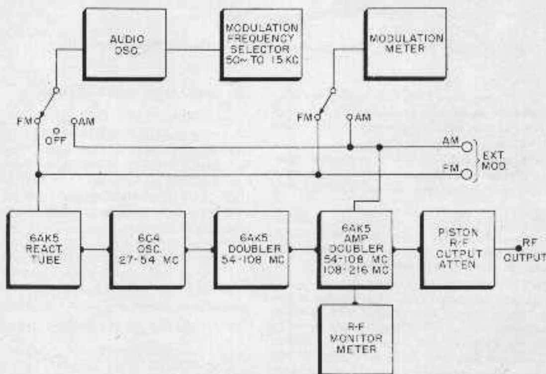
Fig. 1. Basic Elements of 202-B AM-FM Signal Generator
