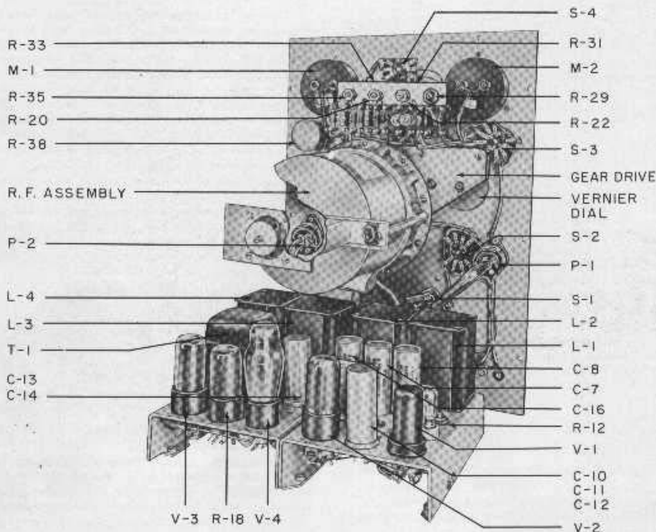
Fig. 5. Rear View of Panel Assembly, Power Supply, and Audio Oscillator
